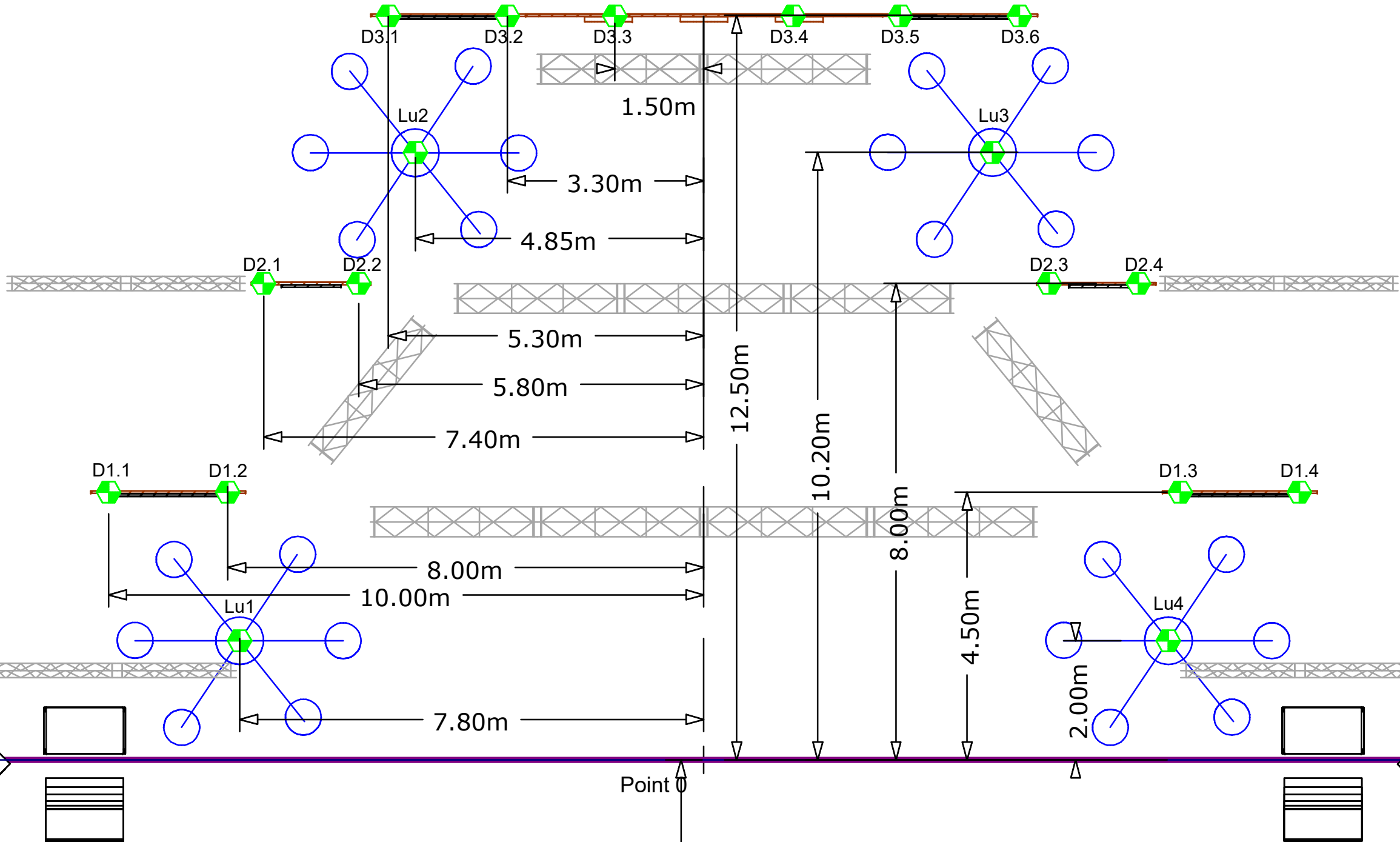
Top view
